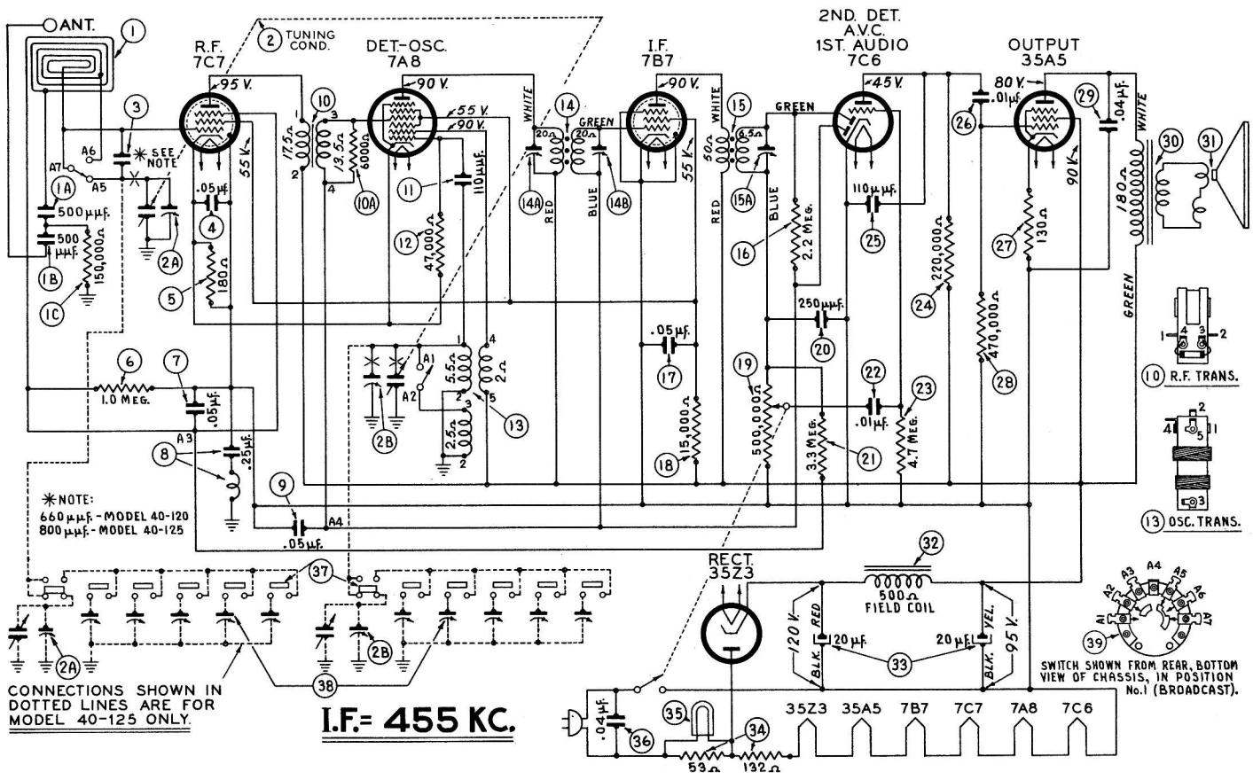
SCHMATIC DIAGRAM MODELS 40-120 & 40-125
